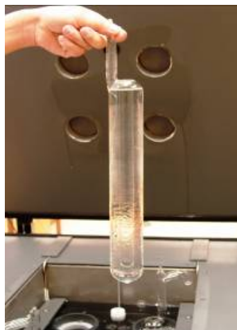
標準及校正實驗所內的水三相點容器 Triple Point of Water Cell in the Standards and Calibration Laboratory
